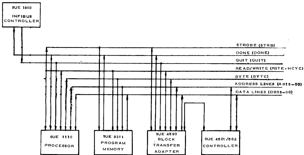
Figure 3-2. Infibus Access Signals
