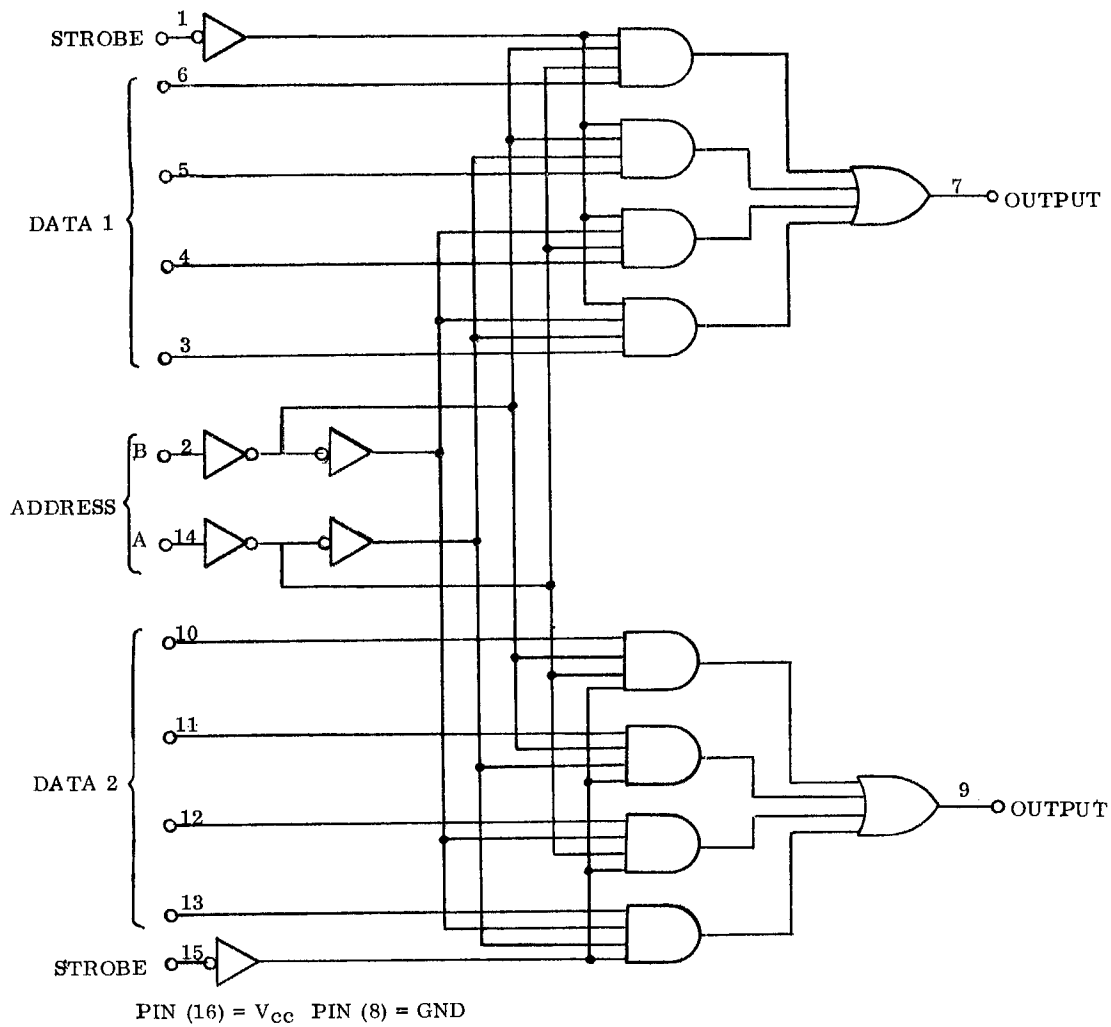
Figure 3-8. Multiplex Logic
