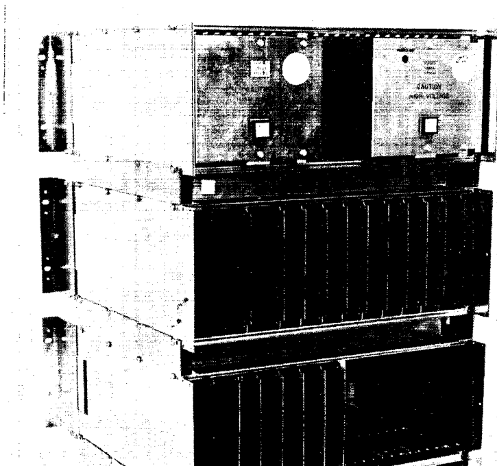
Figure 5-8. Two 7911 Chassis with 5952 Power Supply Note: Placement of cards is for illustration only.
