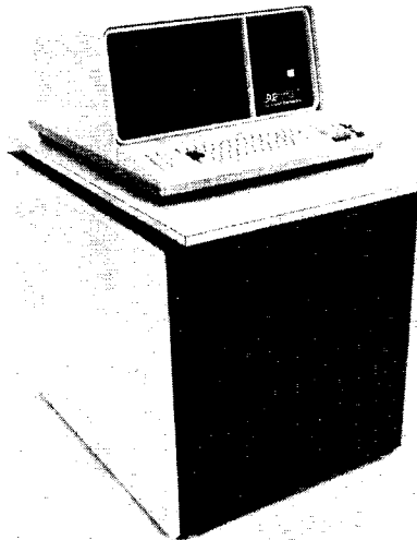
Figure 5-12. Free-Standing System Equipment Cabinet, Model 7932 lo-boy style with optional CRT
