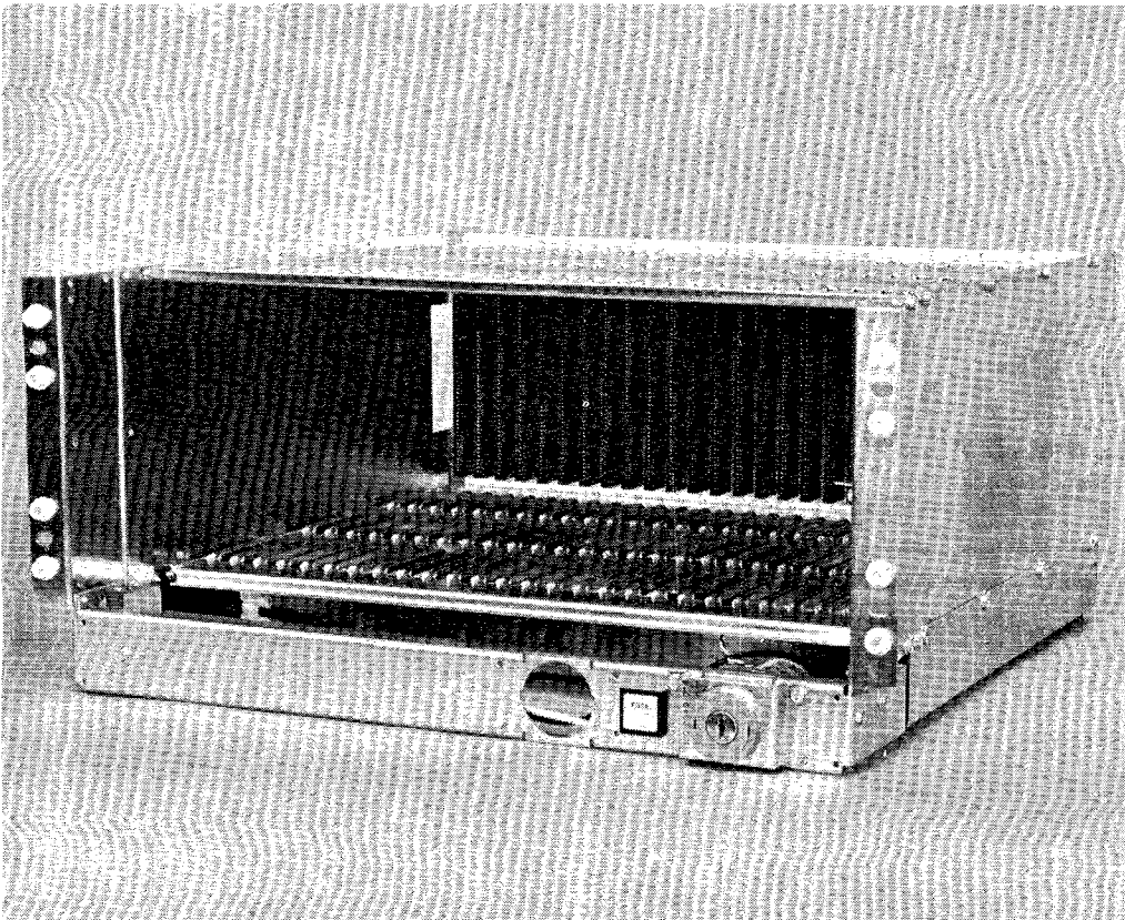
Figure 5-1. Basic SUE Chassis, Model 7910, including 2201 power distribution option
