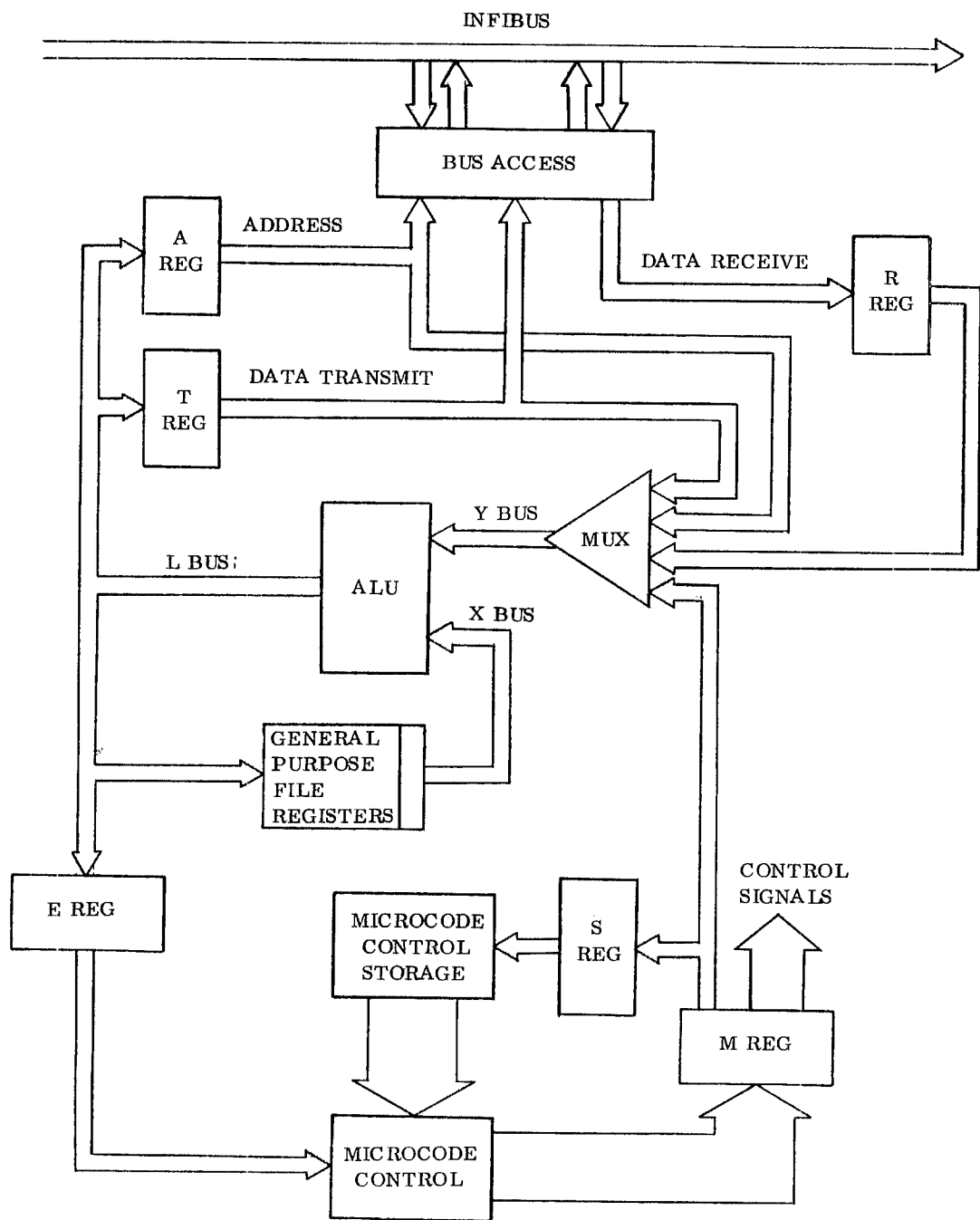
Figure 4-1. SUE Processor Unit Organization
